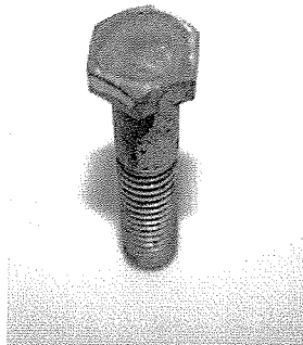
Unretouched photo illustrating the result obtained by placing a drop of diphenylcarbazide solution on the top of a trivalent passivated fastener and placing it in the salt spray cabinet for 24 hours. [Original color photo shows a purple color in the slightly darker shading within the center of the head (about half the diameter) - Ed.]
