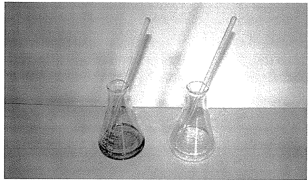
Erlenmeyer flask showing the typical red-violet color of the complex formed between hexavalent chromium and 1,5-diphenylcarbazide. The sample on the left was prepared by diluting and acidifying the condensate from a commercial trivalent passivate obtained from the ASTM B-117 Salt Spray Test and treating the solution with 1,5-diphenylcarbazide at a reduced pH. The Erlenmeyer flask on the right illustrates the result obtained from a control sample that was unpassivated.
